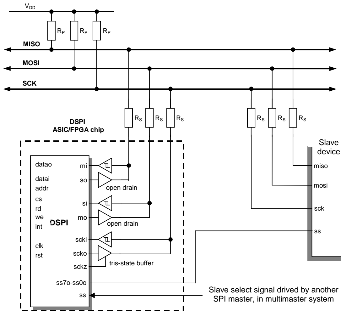
Connection DSPI to global SPI bus
